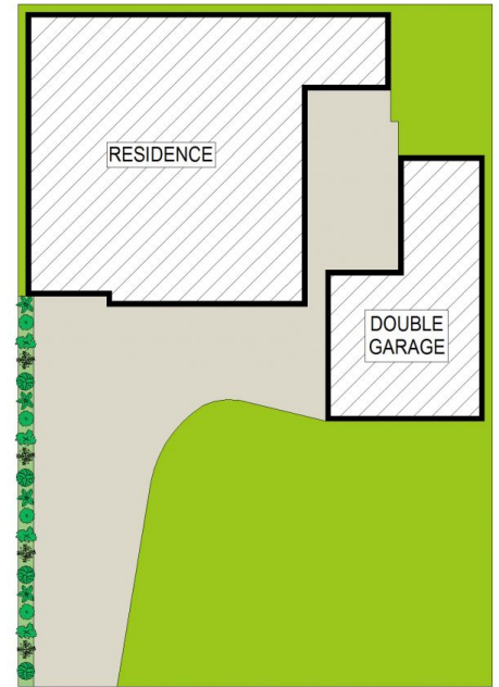
SITE PLAN (NOT TO SCALE) LAND: 563m 2 (approx.)
